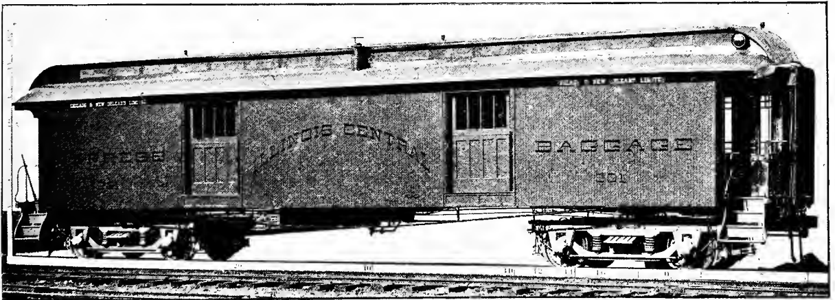
Fig. 140. BAGGAGE AND EXPRESS CAR, ILLINOIS CENTRAL RAILROAD. Length, 50 ft. 8 ins. Capacity, 40,000 lbs. Weight, 48,400 lbs.
